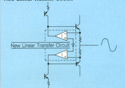
New Linear Transfer Circuit
