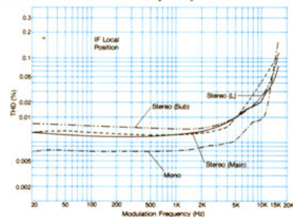
FM THD vs. Modulation Frequency
