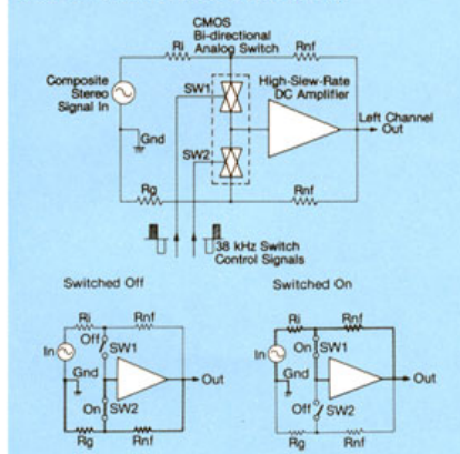
Real-Time Direct MPX Demodulator
