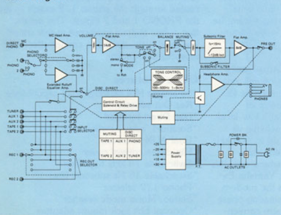
Block Diagram
