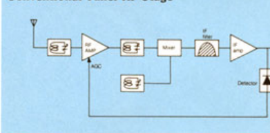
Conventional Tuner RF Stage
