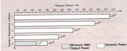
AX-900 Output Power vs. Speaker Impedance
