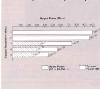
MX-1000 Output Power vs. Speaker Impedance
