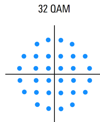
Figure 13 - Wideband HF 32 QAM constellation
