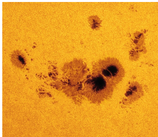
Figure 7 - Sunspots
