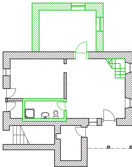
Plan parter
