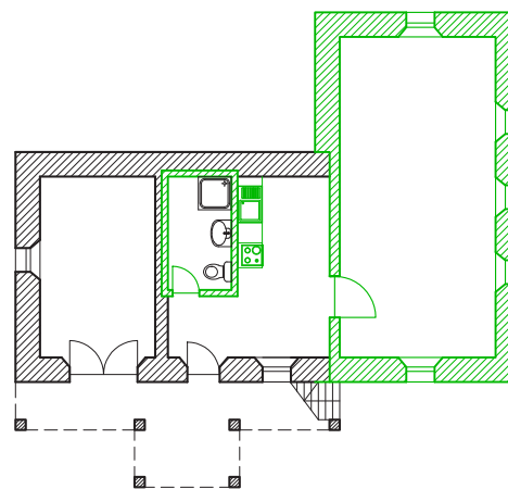
Plan parter
