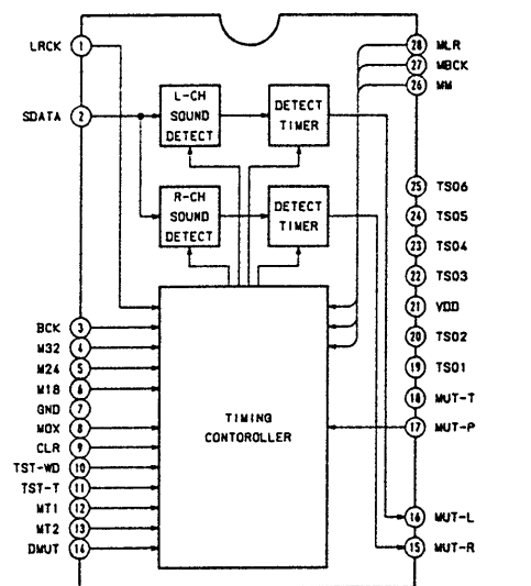
IC203 CXD2553S
