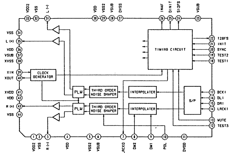
IC202 CXD1244S
